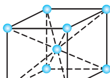
Body-centred
